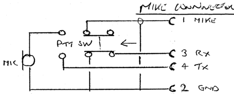
MICROPHONE CONNECTIONS
